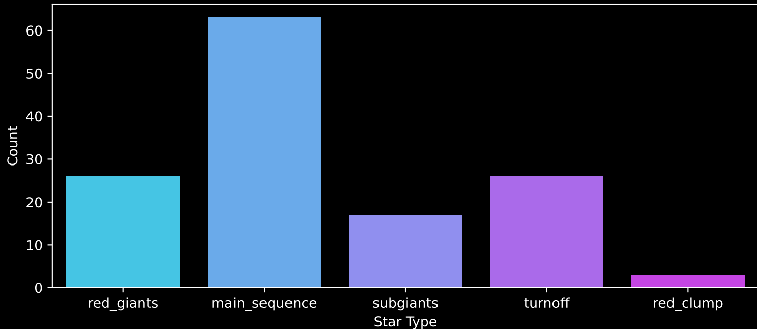
APOGEE DR17 Field: [003-05-O] Count plot of Star Type
