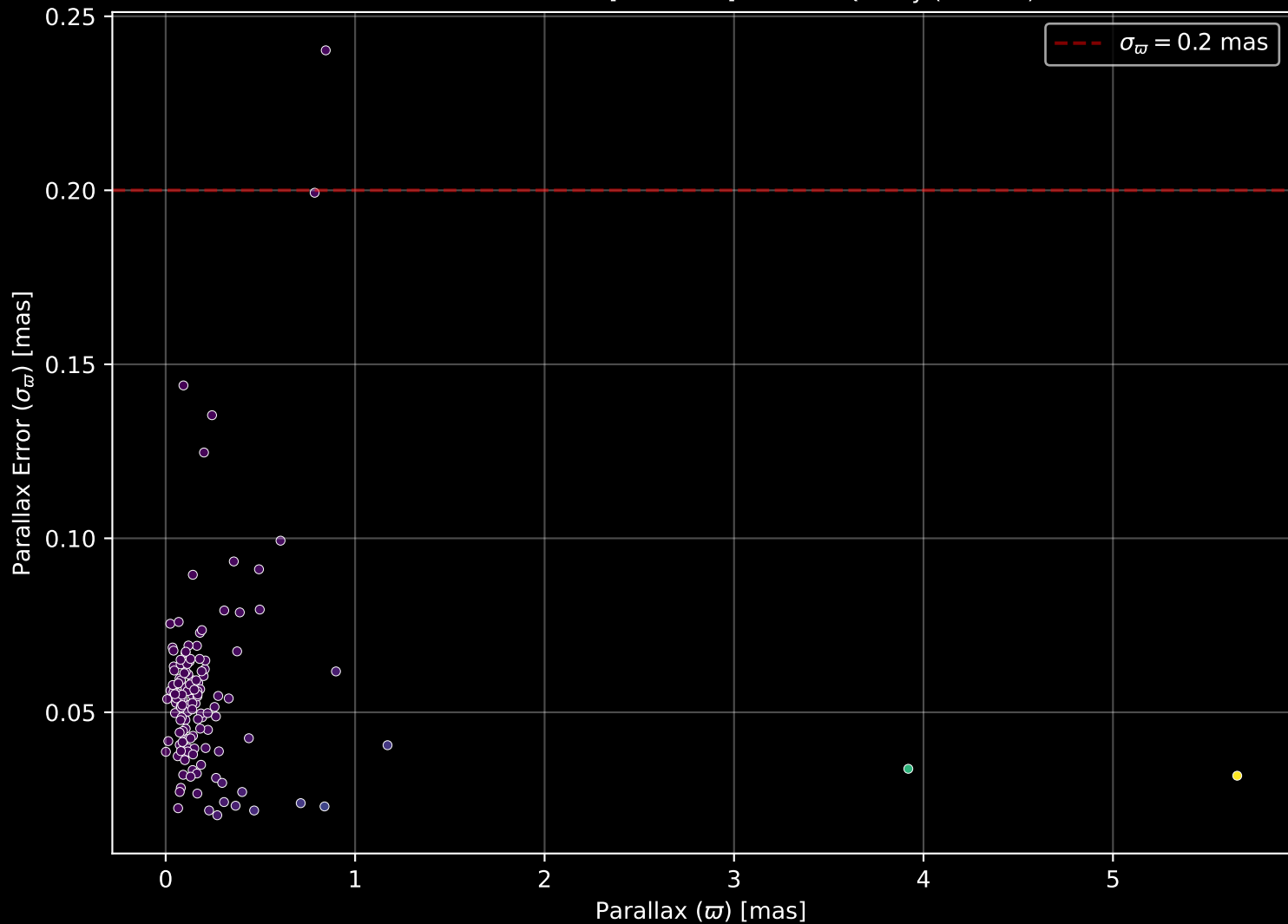
APOGEE DR17 Field: [003-05-O] Parallax Quality (n= 135)
