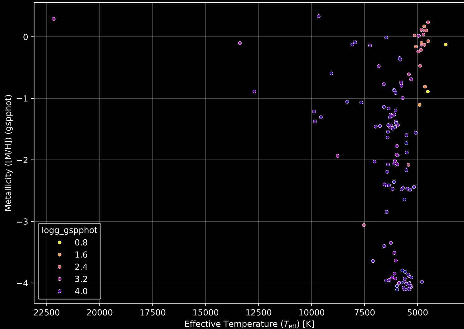
APOGEE DR17 Field: [003-05-O] Stellar Population Parameters (n= 135)
