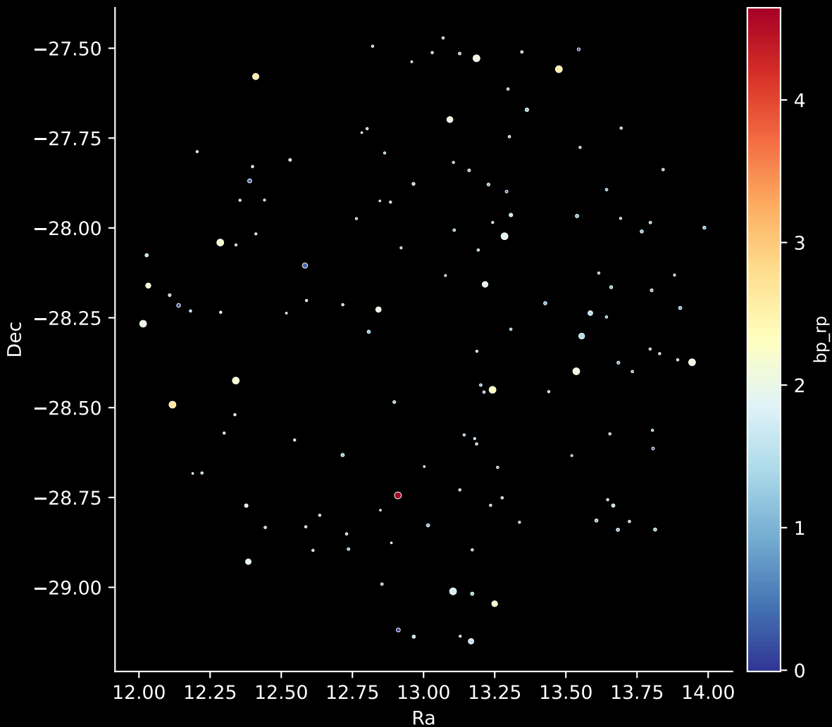
APOGEE DR17 Field: [003-05-O] Stars: 135
