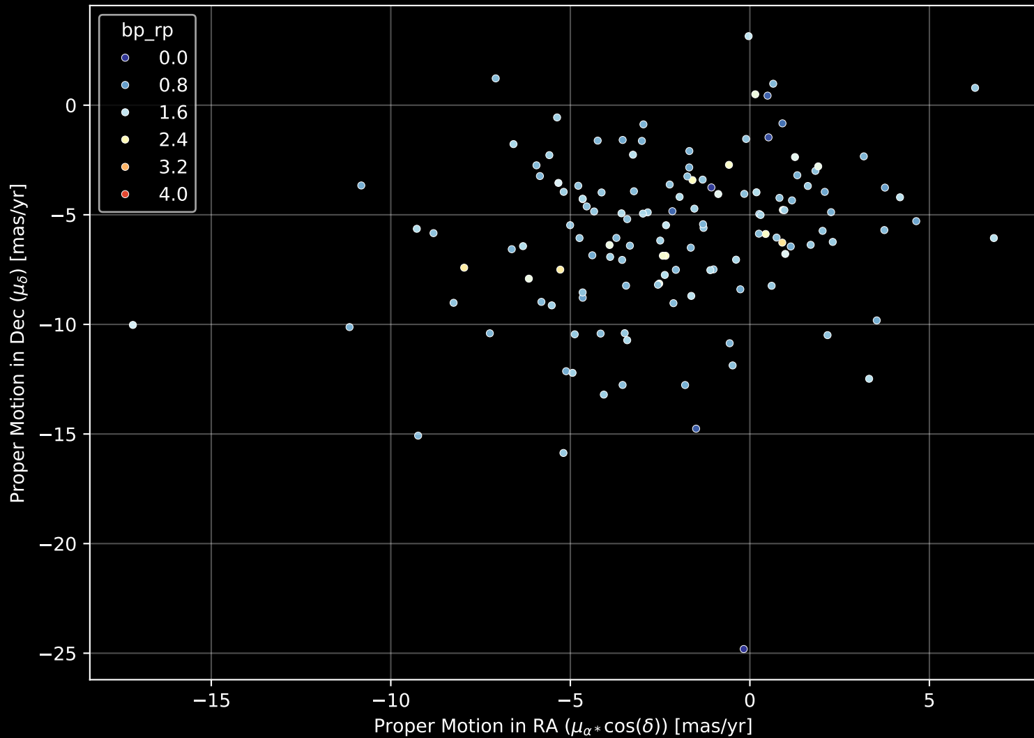
APOGEE DR17 Field: [003-05-O] Proper Motion Diagram (n= 135)
